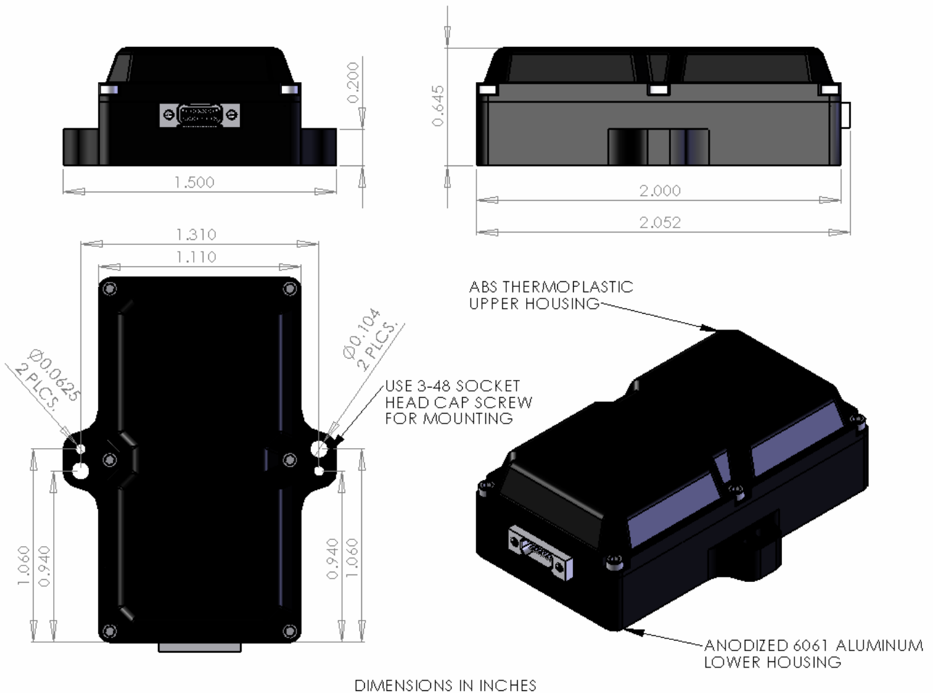
Figure 5 – Physical Dimensions
