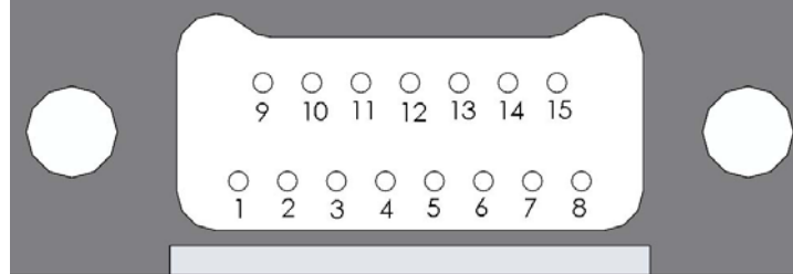
Figure 4 – Omnetics Bi-Lobe Nano interface connector A29100-015
