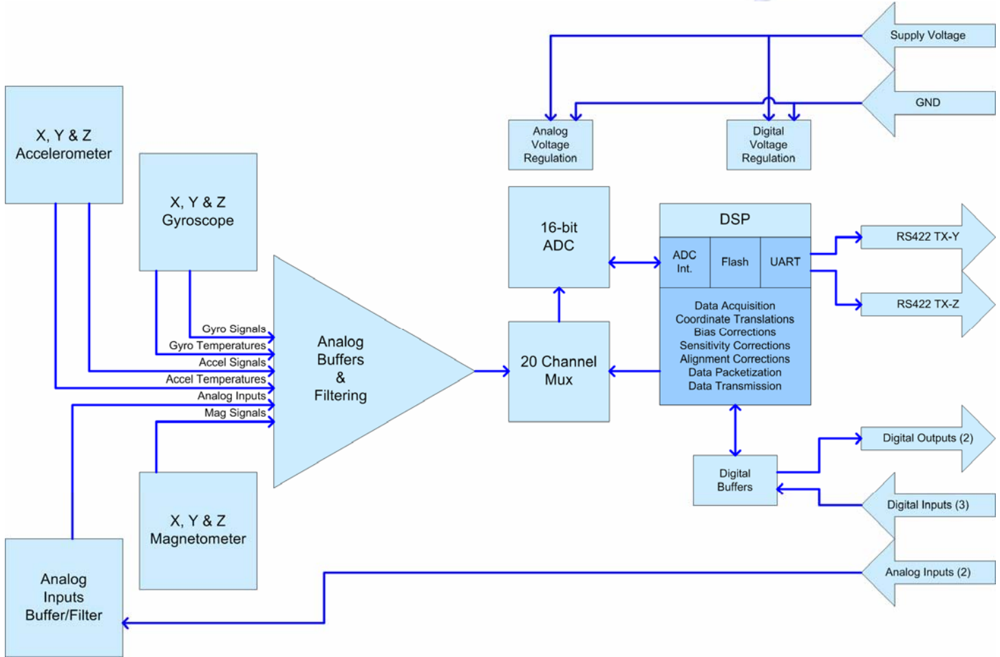
Figure 3 – H3-IMU Functional Block Diagram
